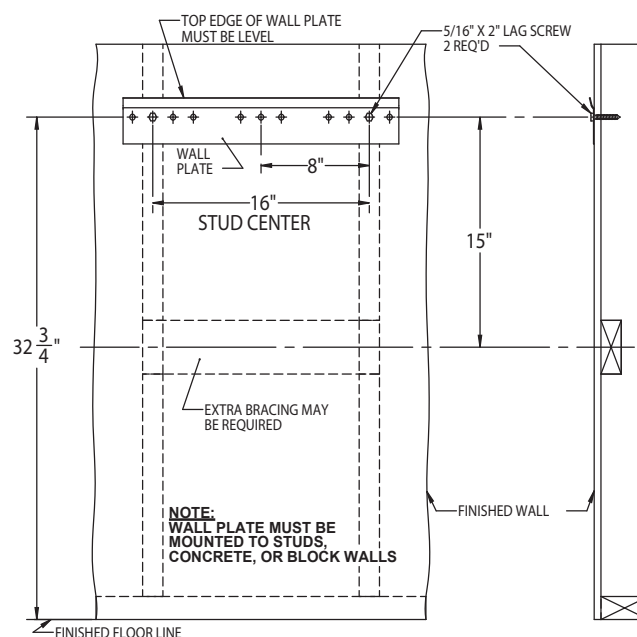
TYPICAL STUD WALL INSTALLATION
